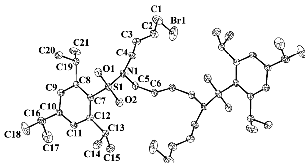
Fig. 1 ORTEP view of 1 after crystallization in a mixture AcOEt–hexane (H atoms are omitted for clarity).
